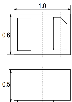
Package Dimensions
